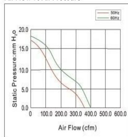
Air Flow vs Air Pressure
