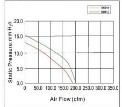
Air Flow vs Air Pressure
