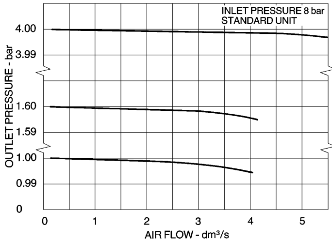
REGULATION CHARACTERISTICS
