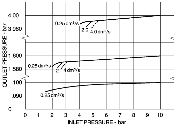
REGULATION CHARACTERISTICS
