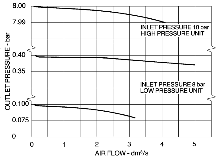
FLOW CHARACTERISTICS
