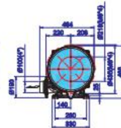
HTB100-203 3-stage
