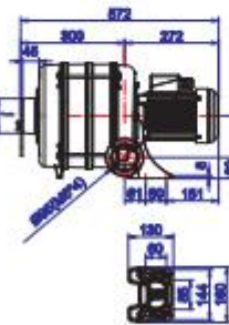
HTB75-104 4-stage
