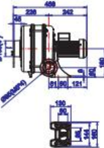
HTB75-053 3-stage
