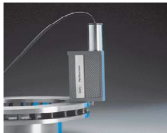
Example: measurement on end face vee
