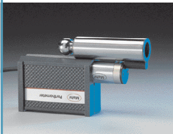
Example: upside down measurement
